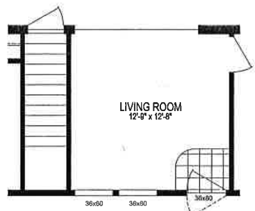
STAIRWELL OPTION (MOD ONLY)
